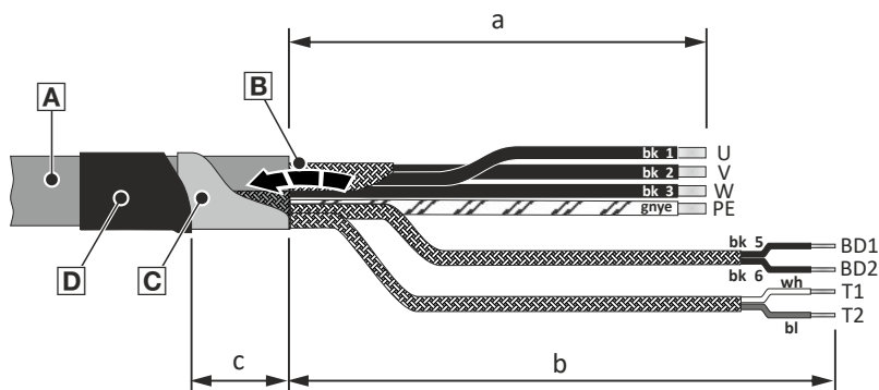
Fig. 10: Cable assembly
