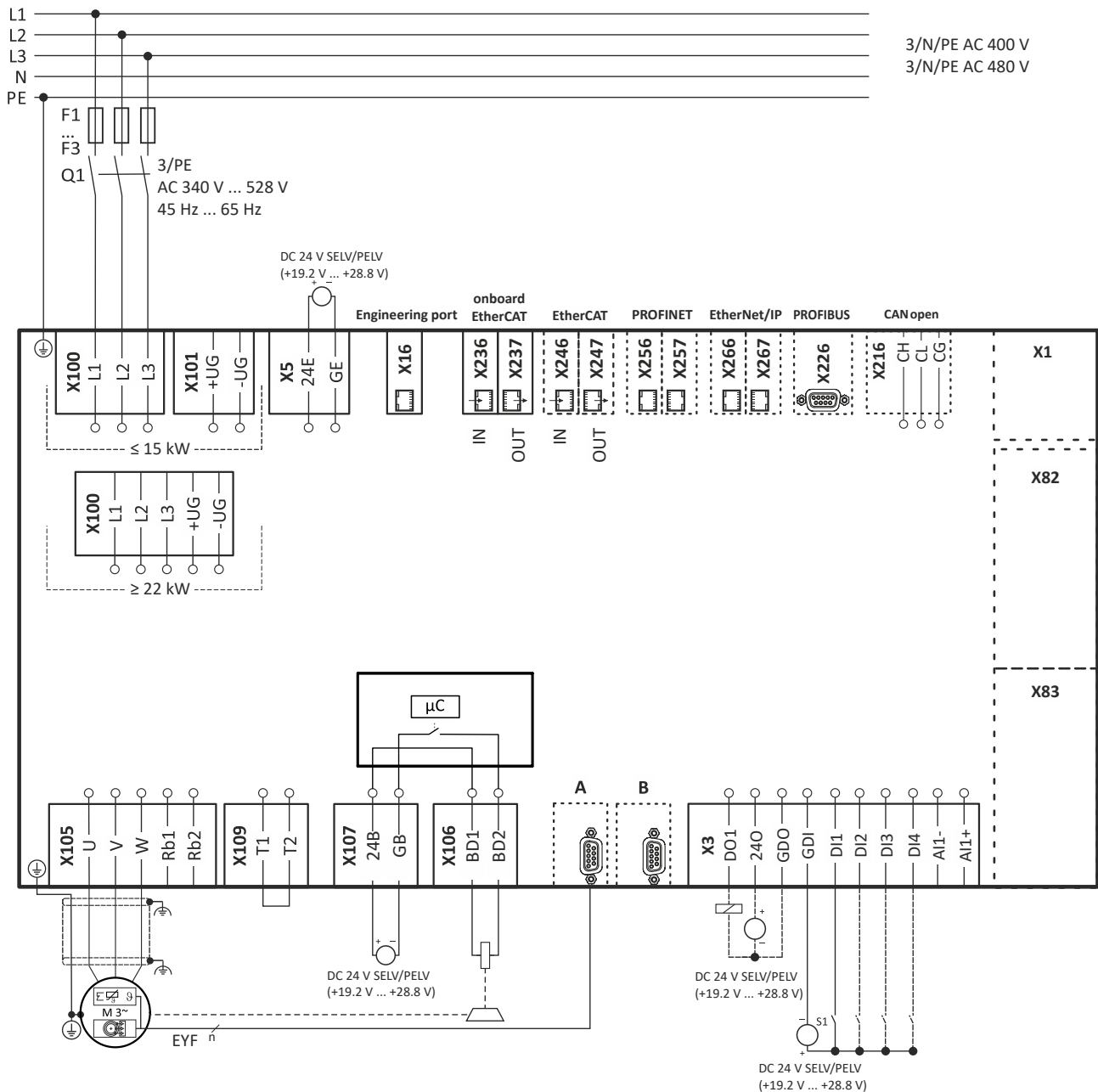
Fig. 5: Wiring example
