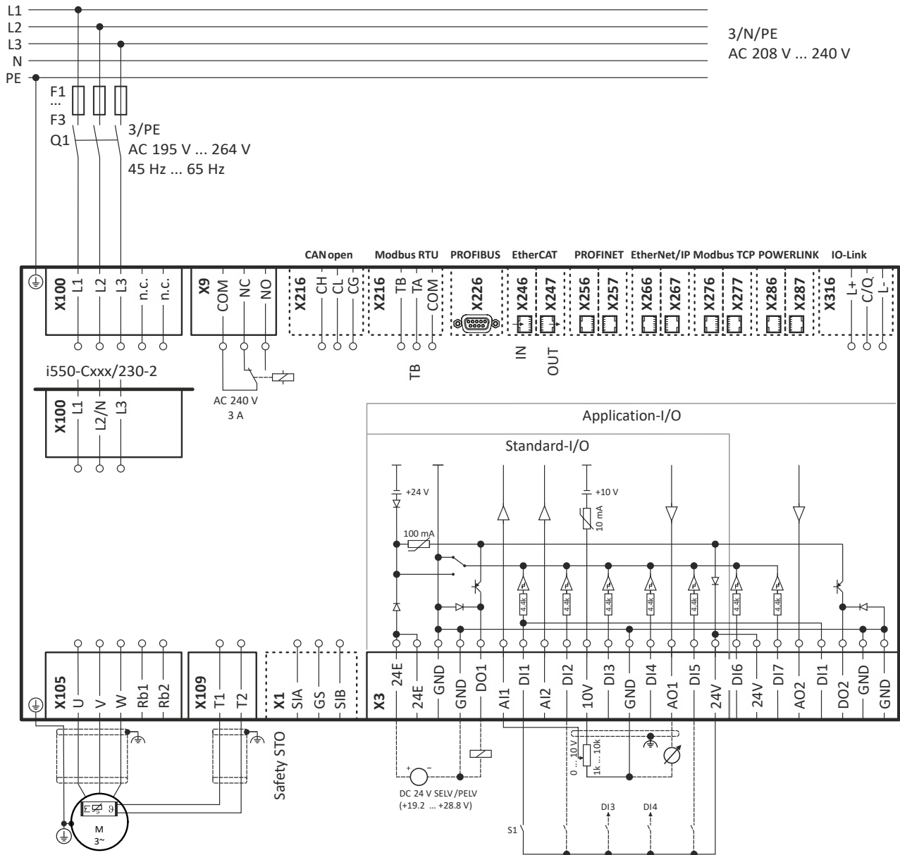
Fig. 5: Wiring example
