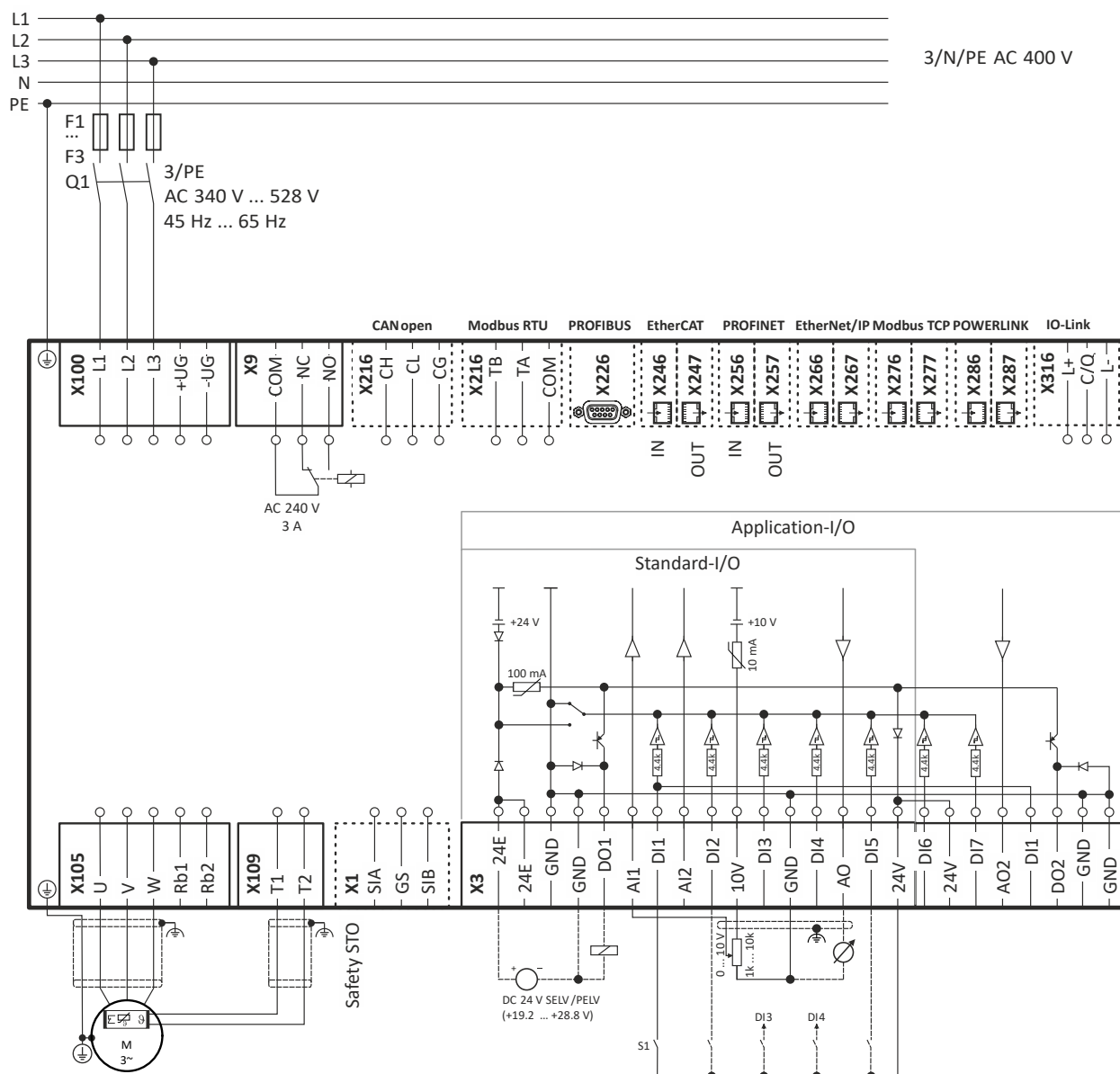
Fig. 6: Wiring example
