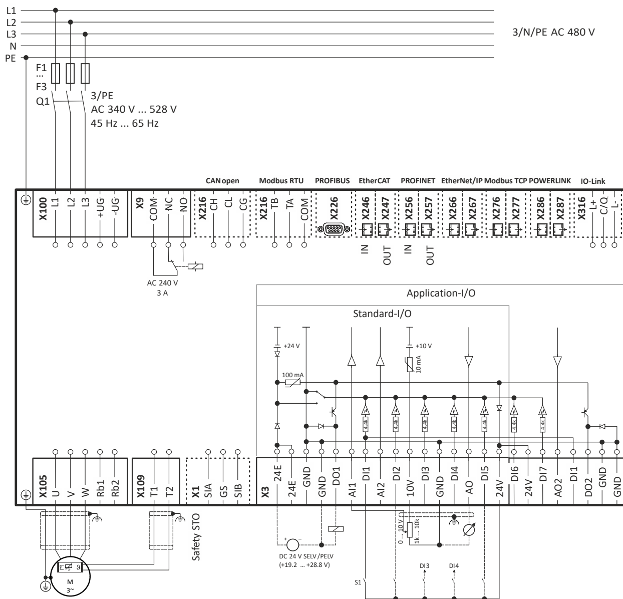
Fig. 7: Wiring example
