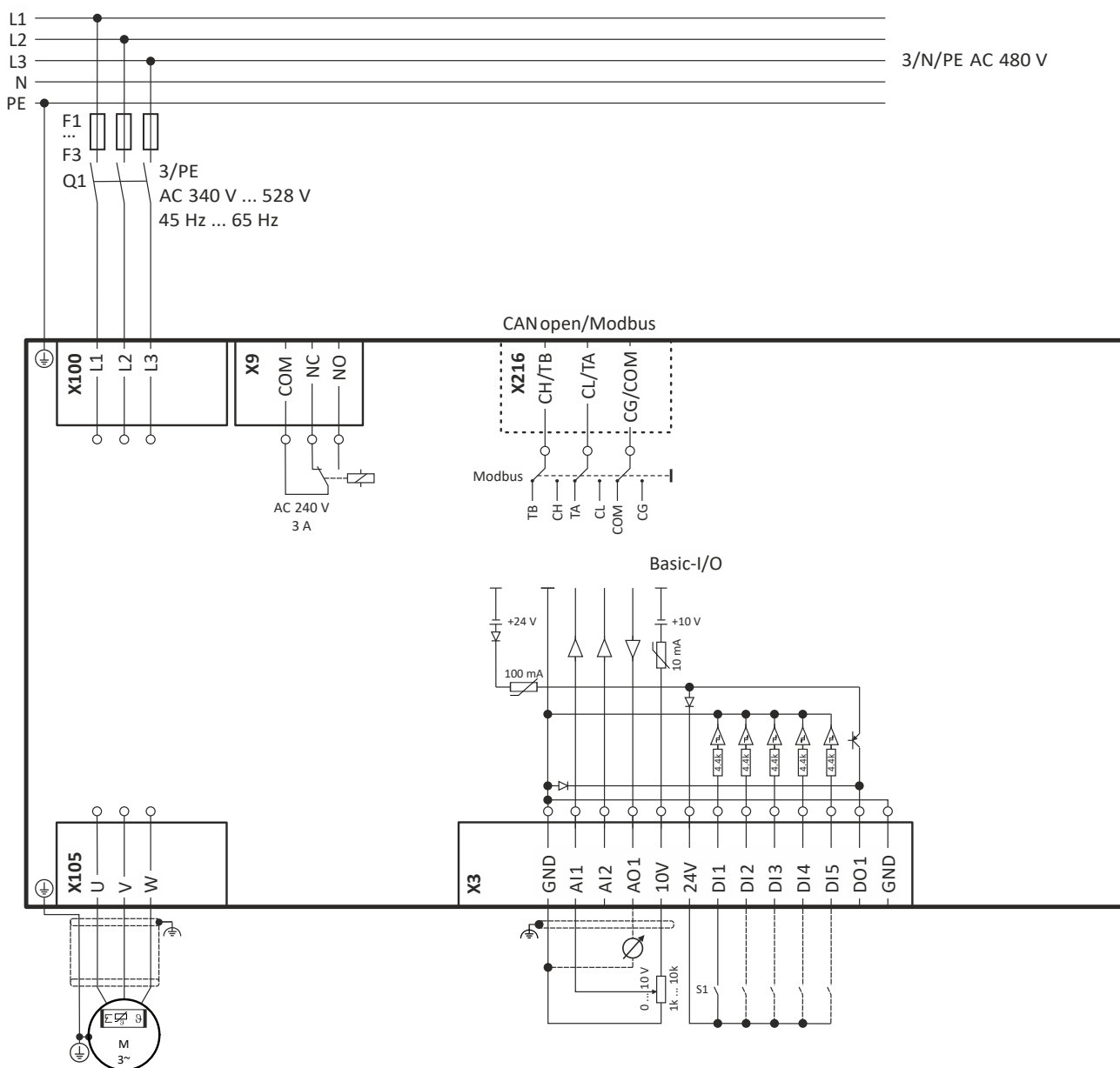
Fig. 6: Wiring example
